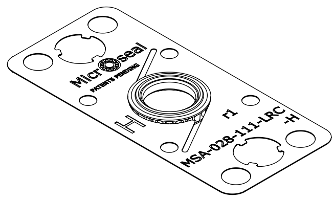
ISOMETRIC VIEW SCALE 3:1
